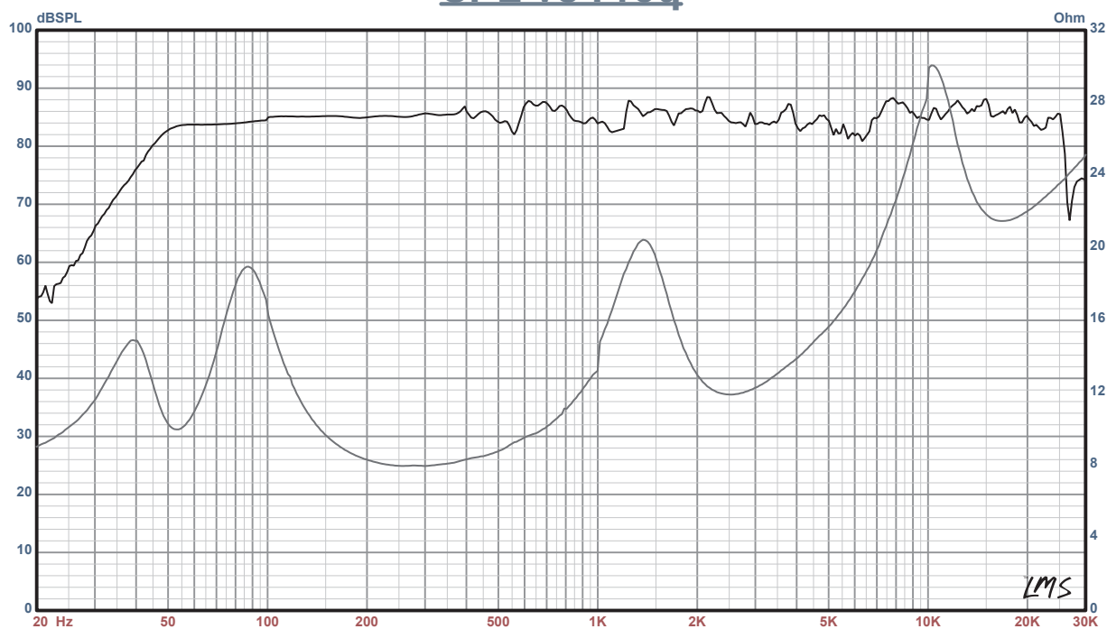
Frequency response Vs impedance diagram (EQ applied)
