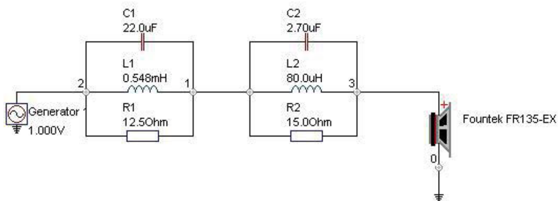
Passive EQ circuit
